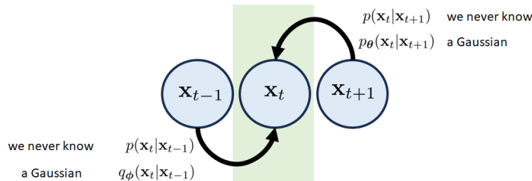
Figure 2.2: The transition block of a variational diffusion model consists of three nodes. The transition distributions p(\mathbf{x}_t|\mathbf{x}_{t+1}) and p(\mathbf{x}_t|\mathbf{x}_{t-1}) are not accessible, but we can approximate them by Gaussians.
